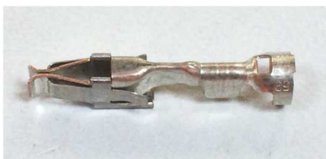
03142253 Cosse Amp JPT 0,5-1,0 Amp JPT contact 0,5-1,0
